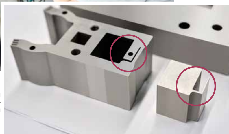
For long, thin contours cut from solid material with wire, the risk of geometry changes due to released internal stresses must be taken into account.
